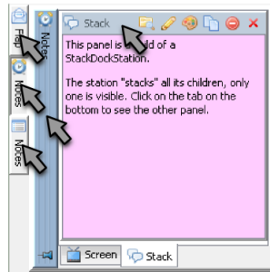
Figure 2: Some DockTitles .
